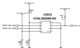
Proxi Sensor
